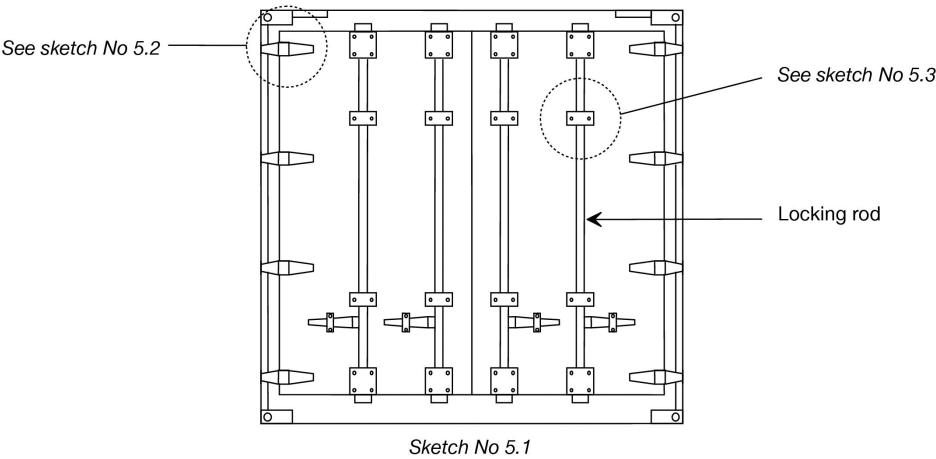
Door—end view
